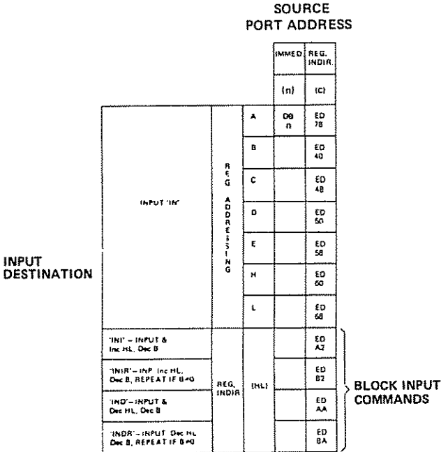
Fig. 4.21: Input Group
