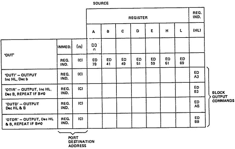
Fig. 4.20: Output Group
