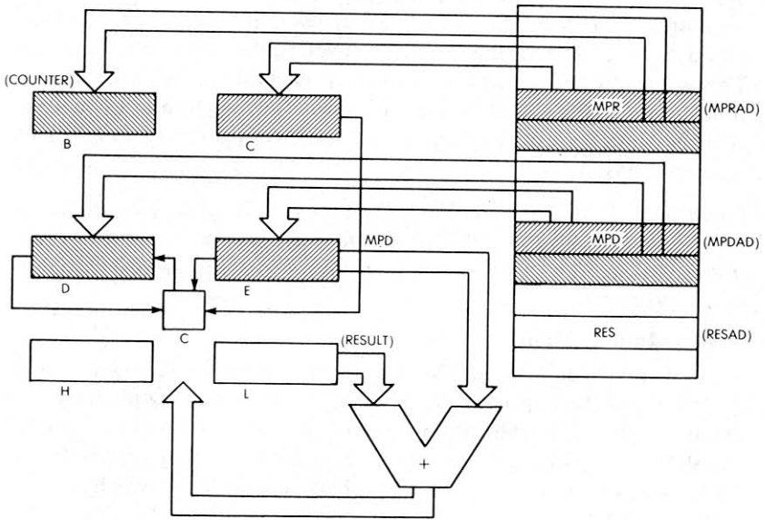
Fig 3.14: 8 × 8 Multiplication—The Registers
