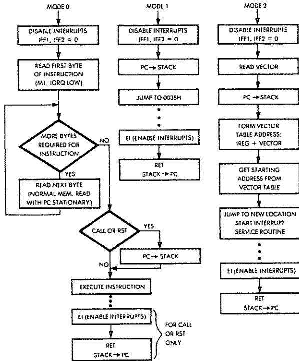
Fig. 6.26: Interrupt Modes
